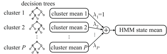
Figure 2: Cluster adaptive training (CAT). Each cluster is represented by a decision tree and defines a basis in expression space. Given a position in this expression space defined by \boldsymbol{\lambda}^{\text{expr}} = [\lambda_1 \dots \lambda_P] the properties of the HMMs to use for synthesis can be found as a linear sum of the cluster properties.
