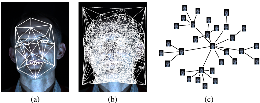
Figure 1: Overview: From a sparse, 37 point AAM (a) the proposed method creates a dense, 1000 point AAM (b) suitable for image synthesis tasks. To achieve the dense registration required to construct the AAM we find a bounded diameter minimum spanning tree on a graph defined on the training images (c). On the digital version it is possible to zoom in to see the individual training images.
