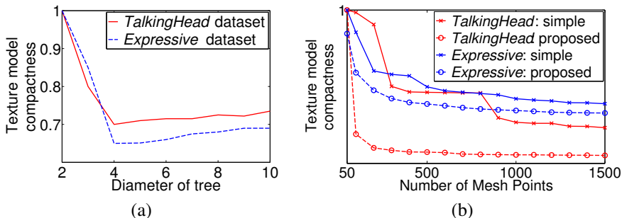
Figure 4: Model compactness for varying parameters. Graphs showing the effect of (a) varying tree diameter and (b) varying mesh density with simple densification (crosses) and the proposed densification (circles). Lower is better.
