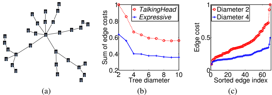
Figure 2: Effects of changing the tree diameter. (a) A minimum spanning tree with diameter D = 10 of the Expressive dataset. (b) Sum of edge costs for a range of minimum spanning tree diameters. (c) Individual edge costs in a minimum spanning tree of diameter 2 (red) and diameter 4 (blue) arranged in ascending order.
