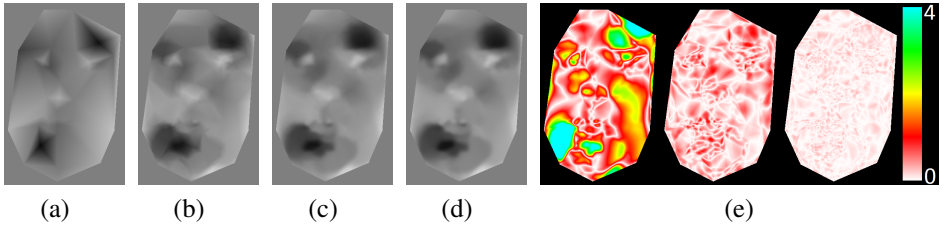
Figure 3: Flow field improvement by AAM densification. (a-c) Approximated horizontal flow fields for one image using meshes with 50, 250 and 1000 vertices respectively, (d) target horizontal flow field, (e) errors between the target flow field and approximations using 50, 250 and 1000 vertices.
